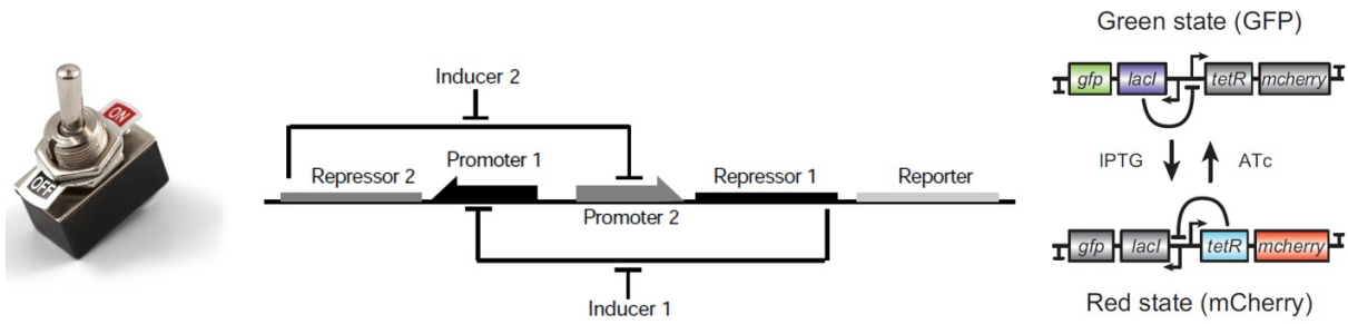
Figure 3: Genetic toggle switch. Left: Common electrical toggle switch with a mechanical lever. The goal here is to construct an analogous switch with two stable states using a genetic circuit in a living cell. Middle: general design of a genetic toggle switch [6]. Right: specific circuit used in this experiment [7]. IPTG and aTc can be used to flip the toggle switch from the green to the red state and vice versa.
